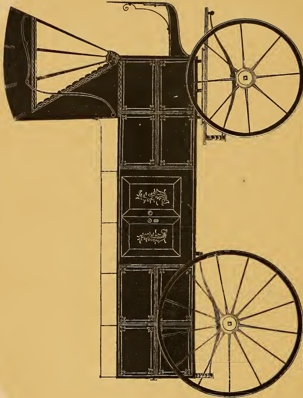
PEDDLER'S WAGON.— \frac{1}{2} IN. SCALE. Engraved expressly for the New York Coach-Maker's Magazine.—Explained on page 110.
